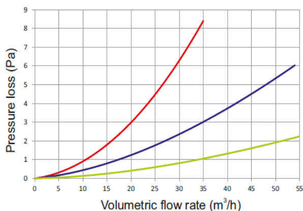
Pressure loss diagram / 1m
