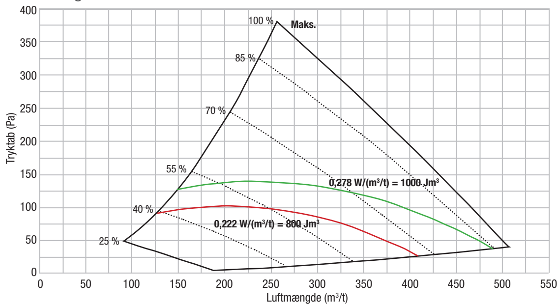
Flowdiagram
